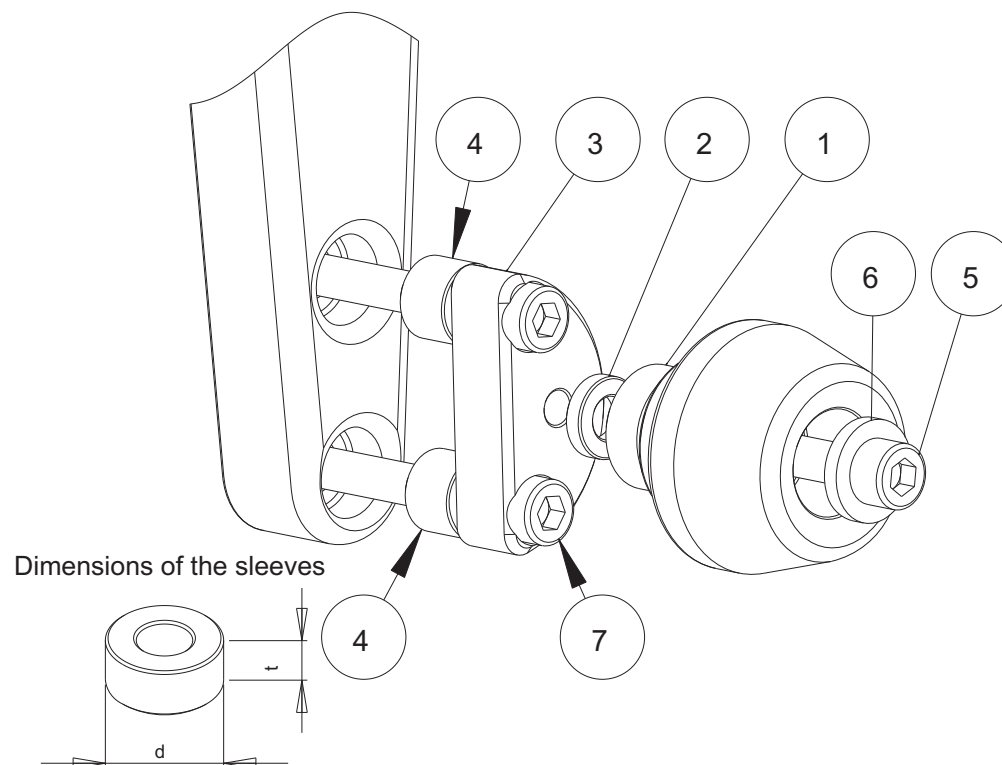
Assembly scheme (both sides)
