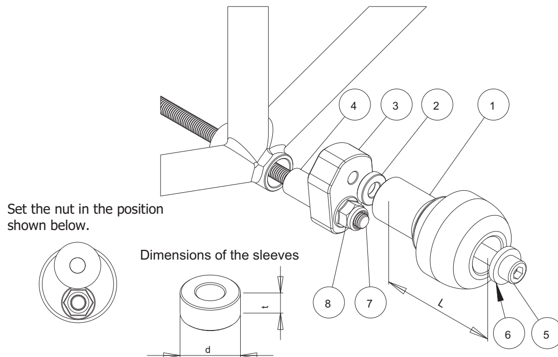
Assembly positions. Left and right sides
