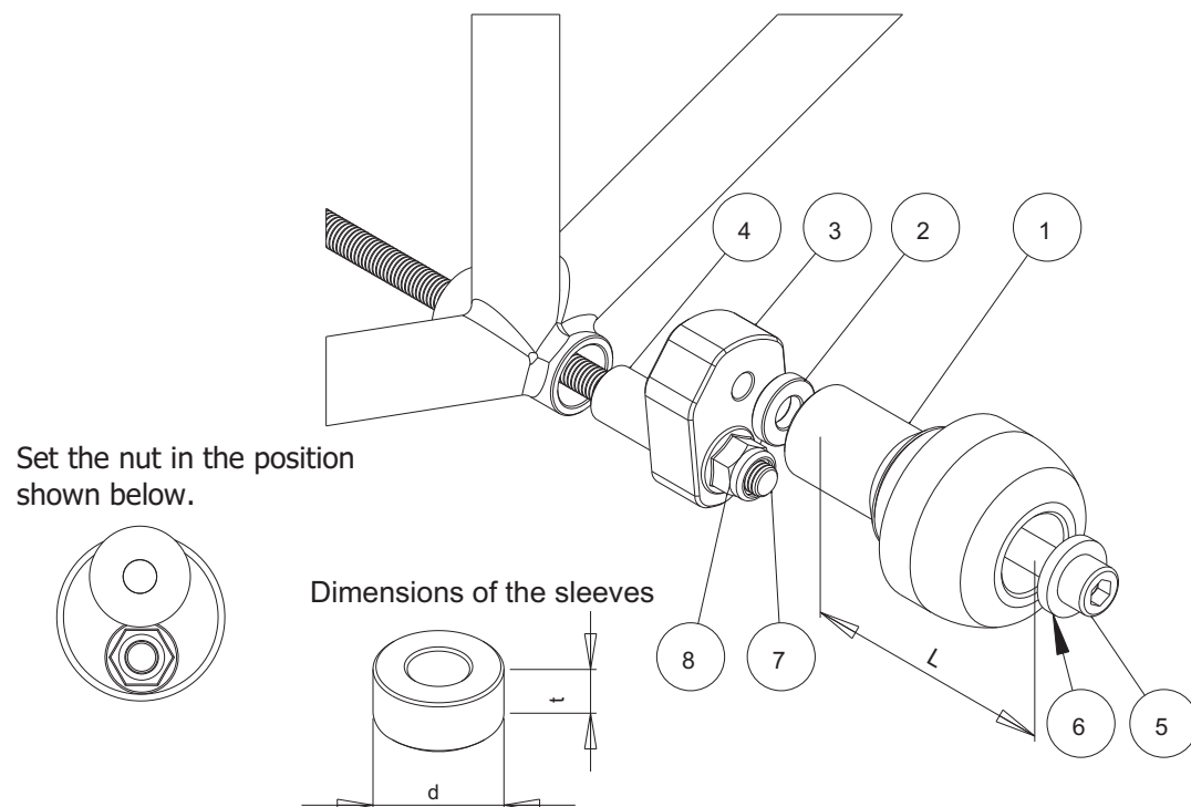
Assembly positions. Left and right sides
